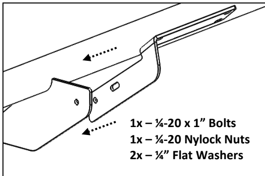
Figure 2: TREADPLATE Bolt-On Center Bracket for Treadplate Step
