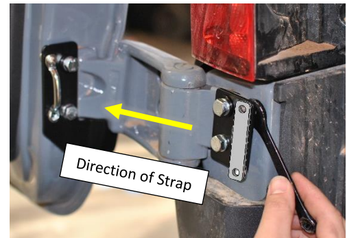
Figure 8: Strap Clamp Install onto Hard Stop Bracket
