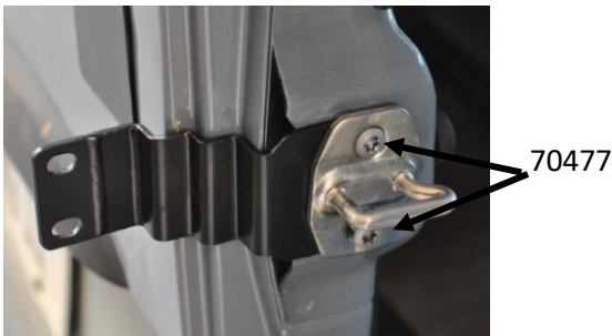
Figure 5: Driver's Inside Door Latch Bracket Installed
