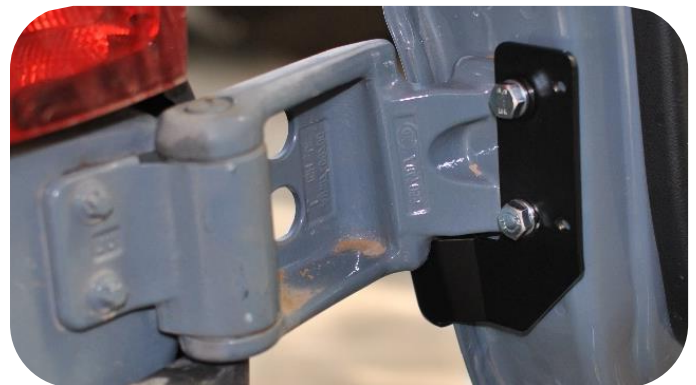
Figure 13: Lower Bracket, Installed Upper Bolt
