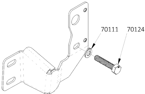
Figure 10: Lower Bracket, Lower Bolt Hardware
