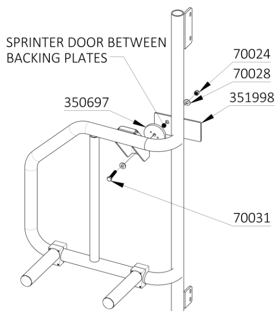
Figure 15: Loosely Installed Center Latch
