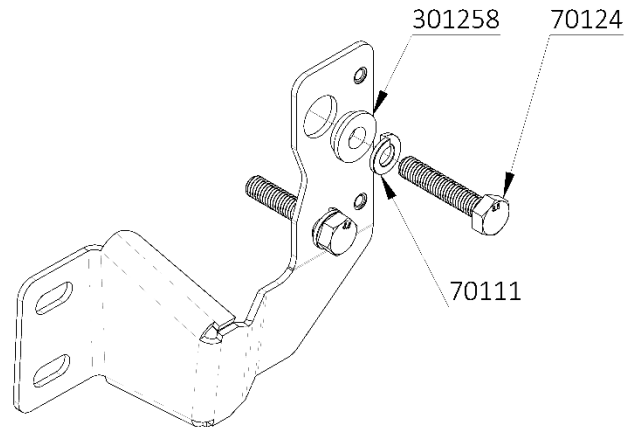
Figure 12: Lower Bracket, Upper Bolt Hardware
