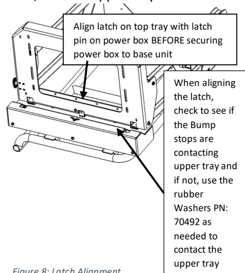
Figure 8: Latch Alignment
