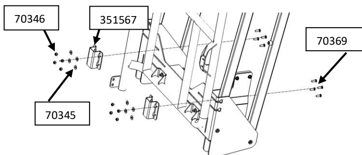
Figure 5: Lower Tray Installation Bracket Bolts
