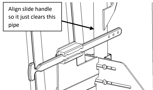
Figure 4: Slide Handle Alignment Image 2
