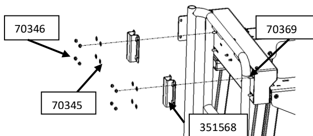
Figure 15: Power Box Installation
