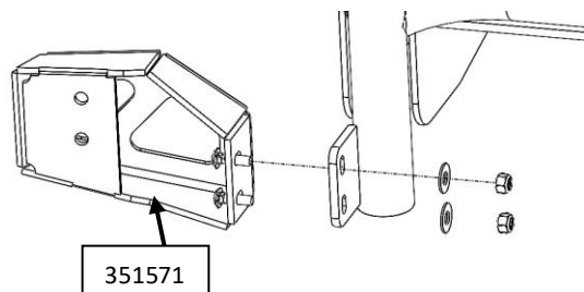
Figure 17: Heavy Duty Lower Hinge Bracket Installation
