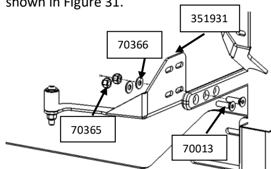
Figure 31: Door Handle Adapter Installation
