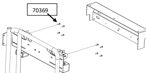
Figure 6: Power Box Carriage Bolt Routing
