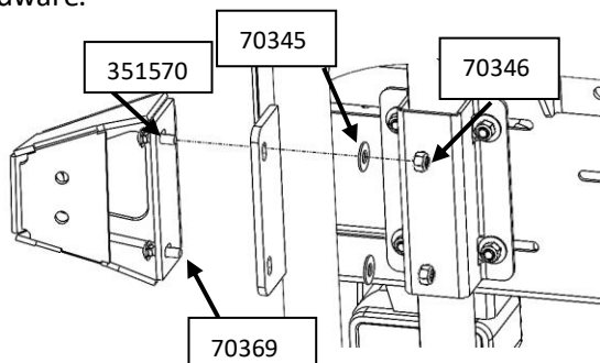
Figure 16: Heavy Duty Upper Hinge Bracket Installation
