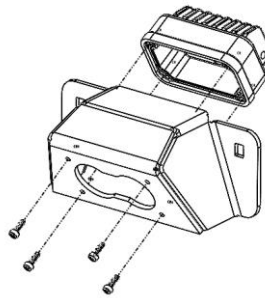
Figure 2: Assembling S2 Light to Light Mount
