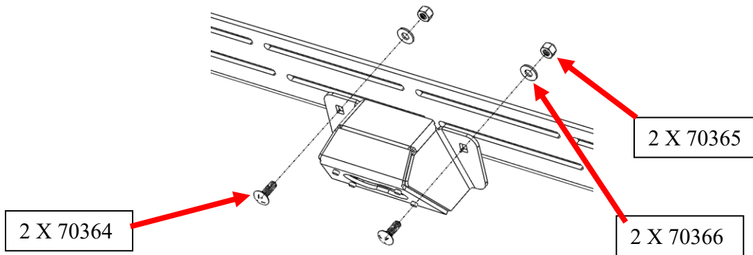
Figure 4: Installing Light Mount along Roof Rack Rail
