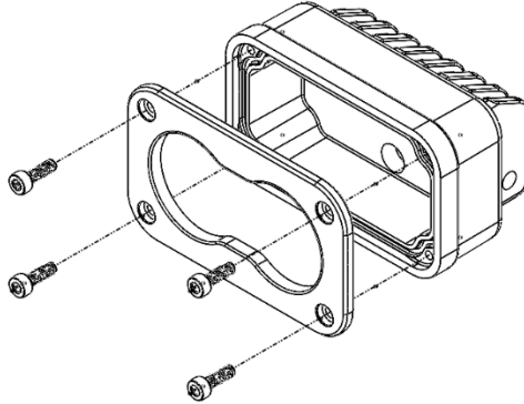
Figure 1: S2 Light Face Plate Removal
