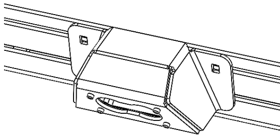
Figure 3: Positioning Light Mount along Roof Rack Rail
