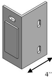
Passenger Angle Bracket PN - 300155
