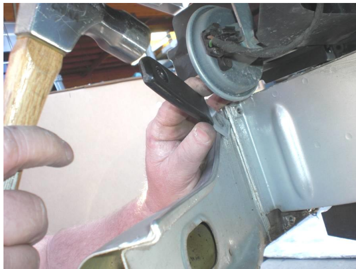
Figure 7: Releasing stock bumper with hammer and putty knife
