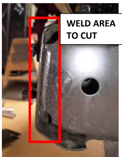
Figure 8a. Crossmember weld before cutting. Figure 8b. Crossmember weld after cutting.
