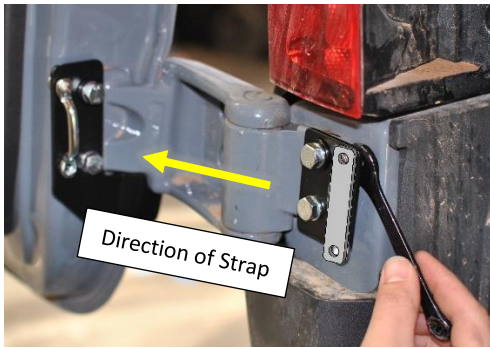
Figure 8: Strap Clamp Install onto Hard Stop Bracket
