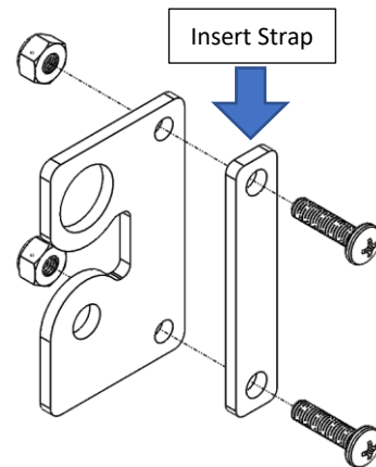
Figure 7: Strap Clamp Assembly
