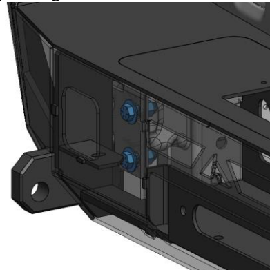
Figure 7: Inside Mounting Locations
