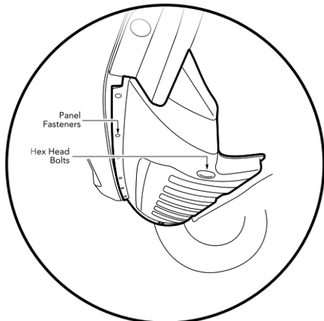
Figure1: Removing plastic push rivets and 5/16" hardware
