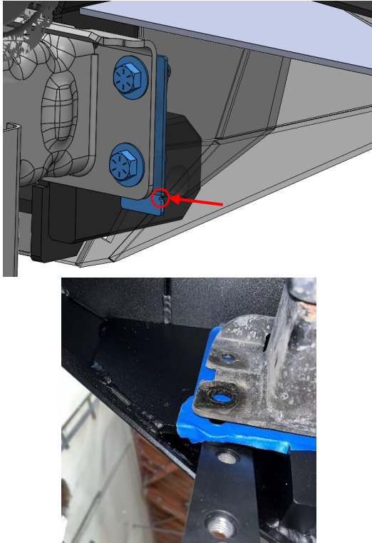
Figure 8: Outside Mounting Locations; Correct Nut Plate Orientation
