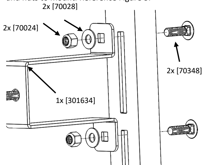
Figure 6: Mounting Tire Bracket
