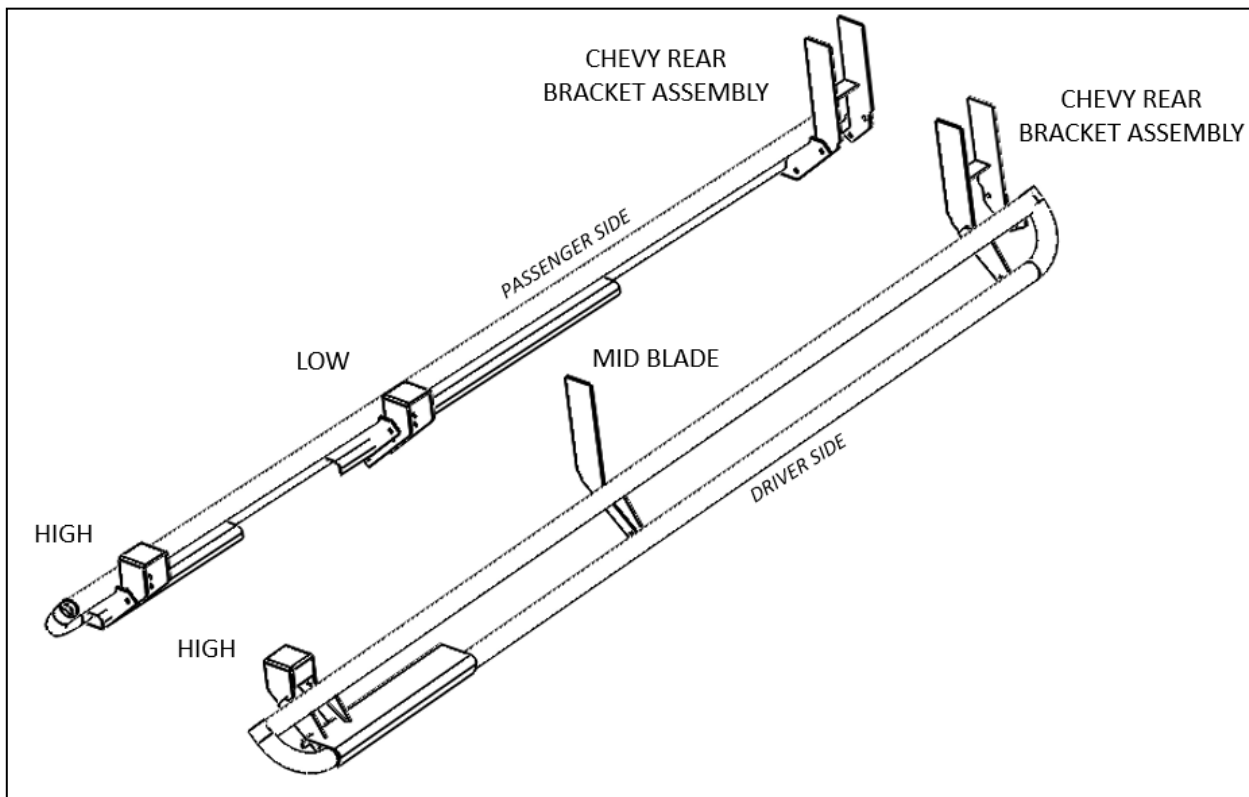
Figure 1. Correct orientation of mounting brackets for Chevy 155 Nerf Bars.
